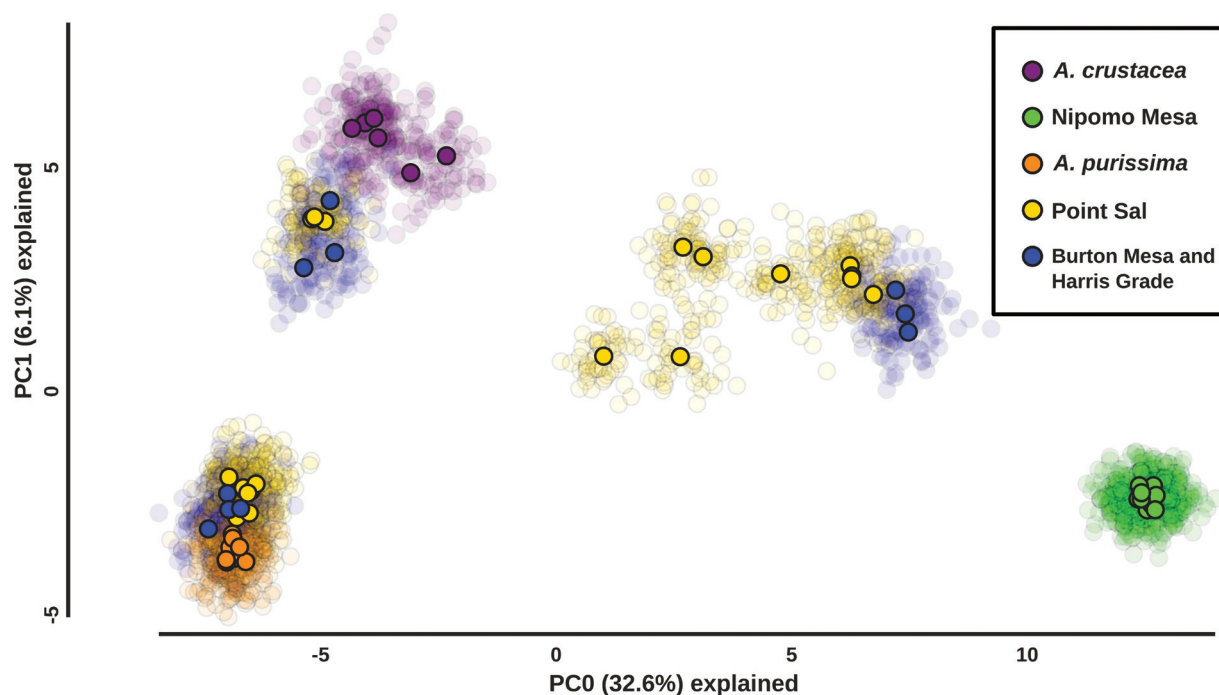
Figure 2. Principal component analysis (PCA) of ddRADseq data with SNPs present in at least 80% of individuals (minimum coverage = 0.8). The figure was generated using the IPYRAD analysis tools (IPYRAD version 0.9.95) and edited in Inkscape version 1.1.2. PC0 is given in the x axis and explains 32.6% of variation in the data, while PC1 in the y axis explains 6.1% of variation in the data. Solid circles are the results of the PCA for a random draw of uncorrelated SNPs for each sample, and the transparent circles are the results of 49 additional PCAs for distinct, independent random draws of uncorrelated SNPs. Missing data was imputed using K-means imputation at K = 4. Samples from the Nipomo Mesa (green), Point Sal (yellow), and Burton Mesa and Harris grade (blue) are color-coded by Sampling location, and samples of Arctostaphylos purissima (orange), and A. crustacea (purple) from control/nonfocal populations are color-coded by taxonomic identity.
