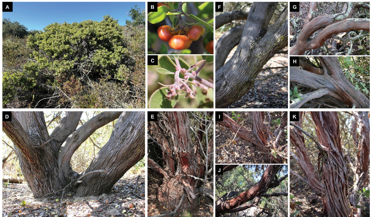
Figure 7. Diagnostic photographs of Arctostaphylos nipumu (Nipomo Mesa, San Luis Obispo County, CA) and A. rudis (Burton Mesa, Santa Barbara County, CA) A A. nipumu in situ, maritime chaparral habitat B depressed fruit of A. nipumu C nascent inflorescence, with leaf-like bracts proximally grading to scale-like bracts distally D A. nipumu , lacking a burl at the base of the stem E A. rudis with a pronounced burl at the base of the stem F–H gray to reddish-gray, thinly shredding bark of A. nipumu I–K pronouncedly red to reddish-gray, coarsely and variably shredding bark of A. rudis .
